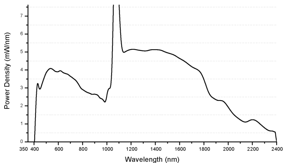
8W SC-OEM Typical Spectrum(4MHz)
