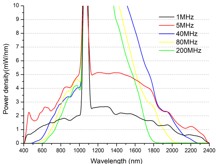
8W SC Pro Typical Spectrum
